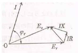
Leading power factor: E_r > E_s
