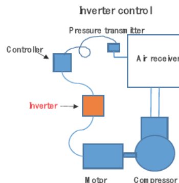
Inverter control outline
