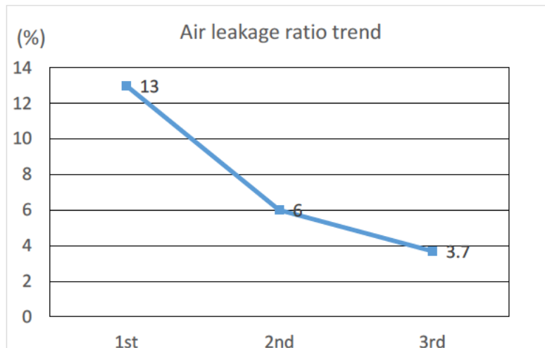
Figure 3 Trend of air leakage ratio for 1 year
