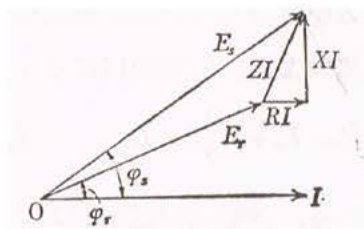
Lagging power factor: E_r < E_s
