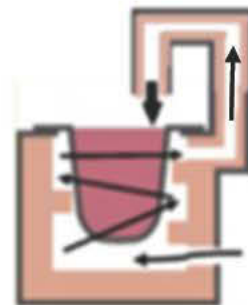
Spiral flame flow & U-turn chimney
