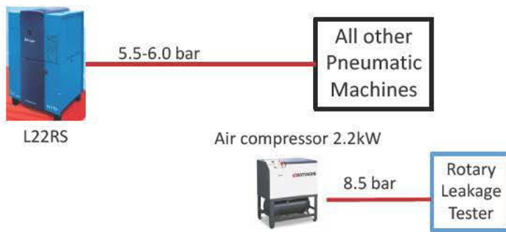
Figure 2 Installation of high pressure air compressor
