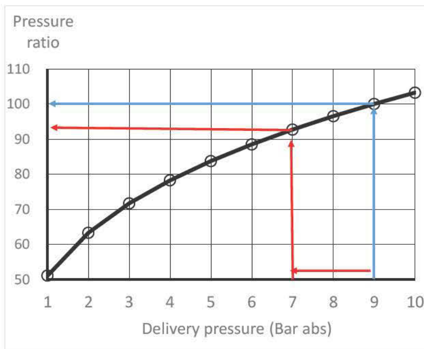
Figure 3 Relationship between delivery pressure and power consumption of compressors
