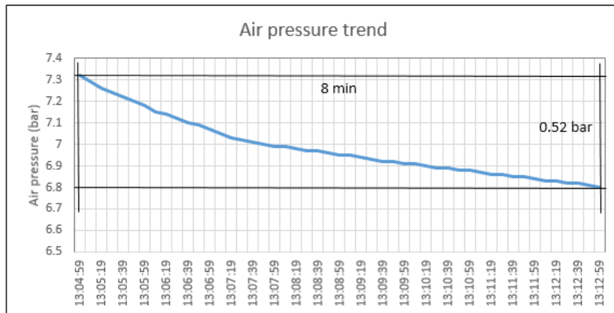
Figure1 Measurement of air pressure reducing trend at outlet of compressor during no air use in plant.
