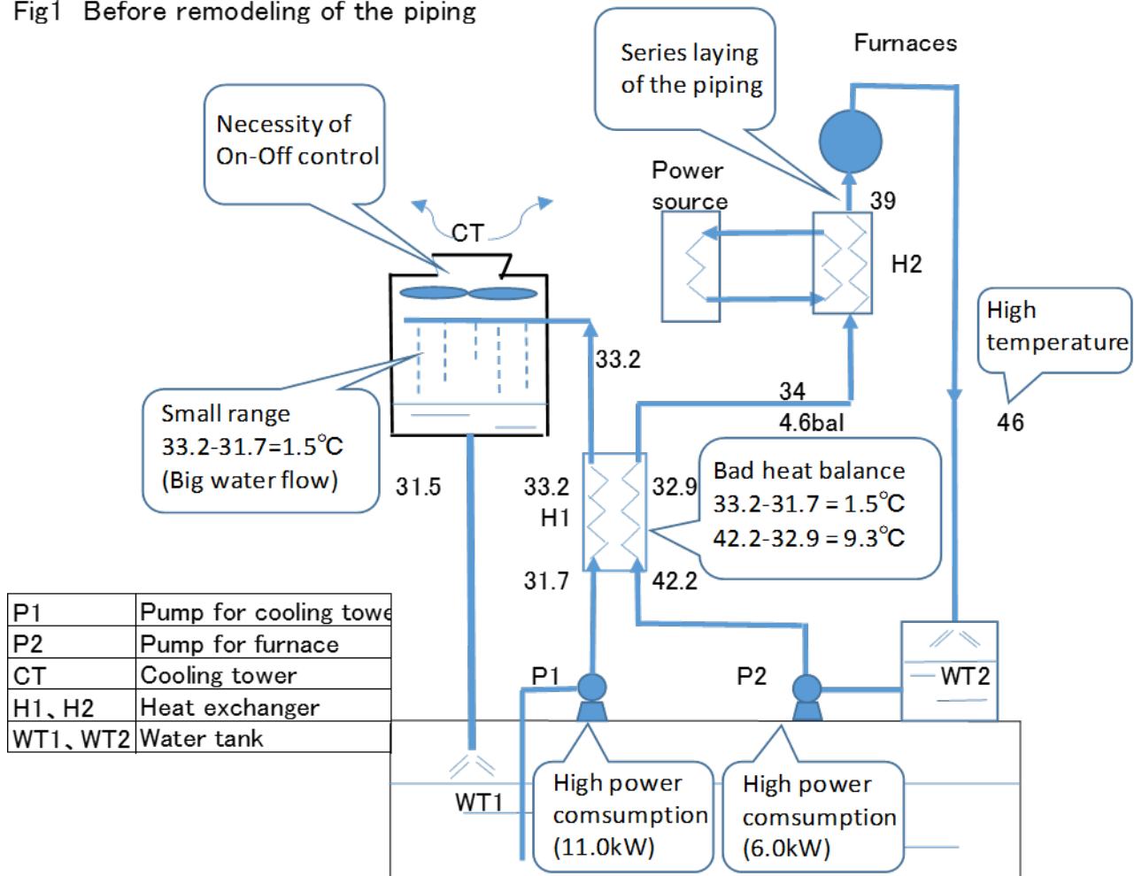
Fig1 Before remodeling of the piping
