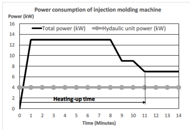
Figure 3 Power consumption of injection molding machine
