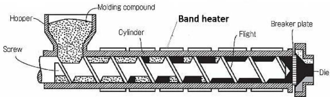
Figure 1 Section of heater cylinder of plastic injection molding machine
