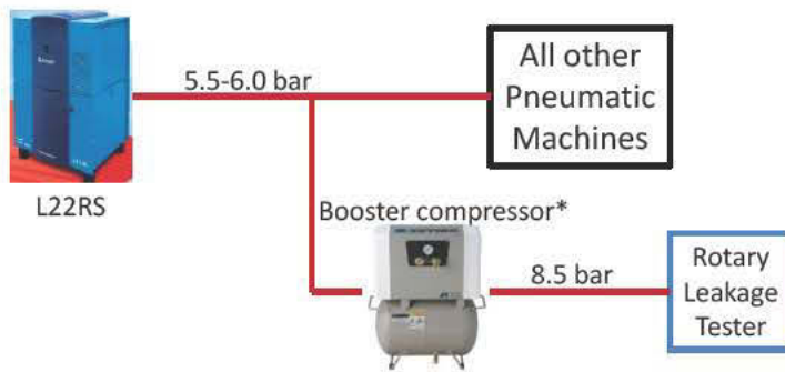
Figure 1 Installation of booster compressor
